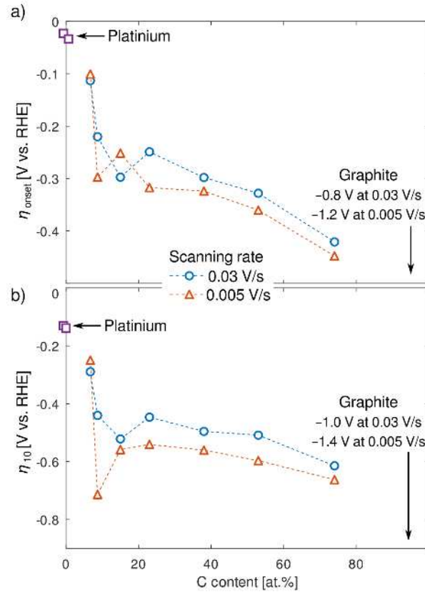
Figure 11: Onset overpotential \eta_{\text{onset}} and the overpotential that results in the current density of 10 \text{ mA/cm}^2 - \eta_{10} . The values were read from the linear voltammetry curves presented in Fig. 9
