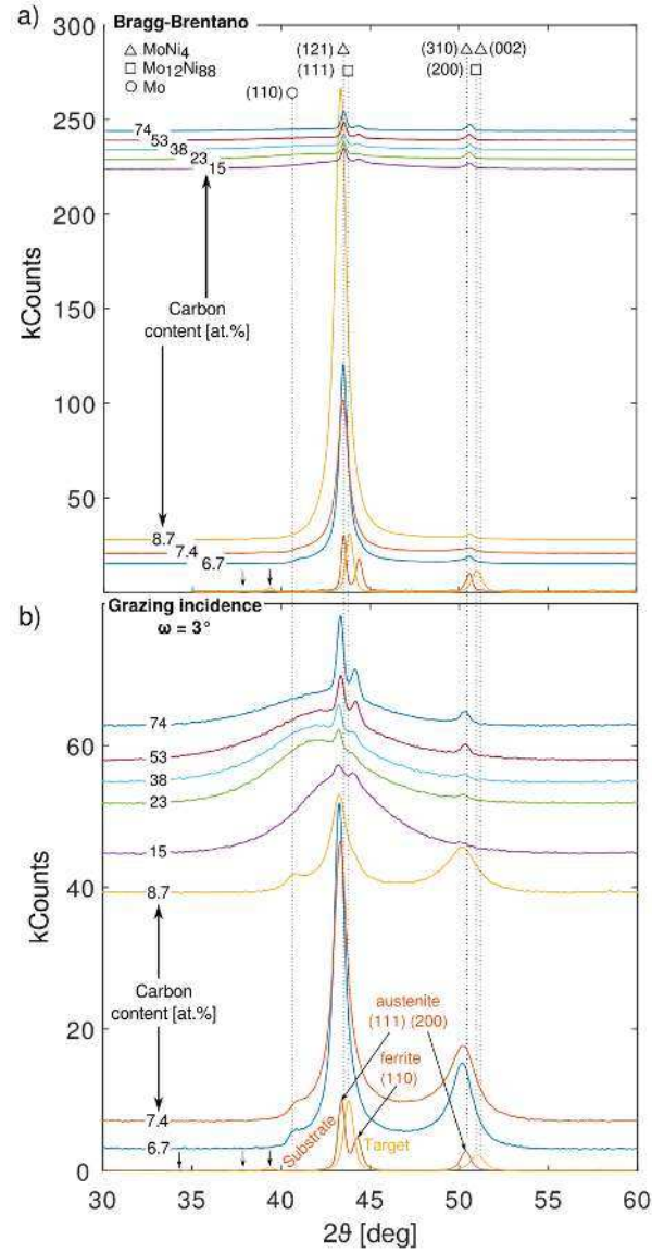
Figure 4: X-ray diffraction patterns of substrate material (316L steel), target ( \text{Ni}_{80}\text{Mo}_{20} alloy), and NiMo-C coatings with increasing carbon content. The patterns recorded in a) Bragg-Brentano geometry and b) low constant incidence angle.
