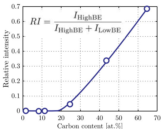
Fig. 4. The relative intensity (RI) of the high binding energy (BE) component in the C1s spectra for the coatings with increasing carbon content.
