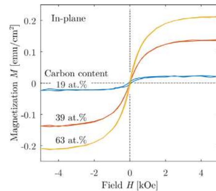
Fig. 6. In-plane magnetisation curves for NiCr-C films with various carbon content.
